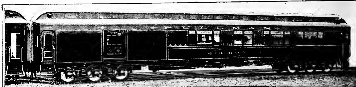
Fig. 134. COMBINATION SMOKING, BARBER SHOP, BATH ROOM AND BAGGAGE CAR. Exhibited at World's Columbian Exposition, 1893, by Pullman's Palace Car Company. (Plan is shown in Fig. 181, interior in Fig. 133.)
